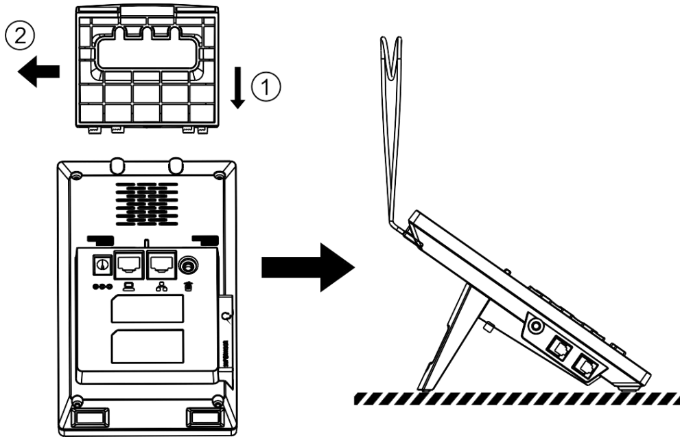
Figure 1 - Bracket installation
